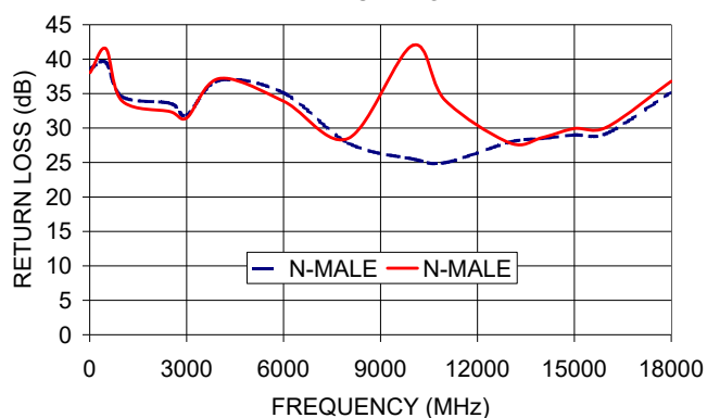
APC-10FT-NMNM+ RETURN LOSS
