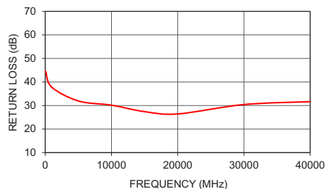
ANNEF-50K+ RETURN LOSS
