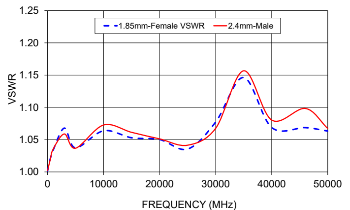
185F-24M+ VSWR
