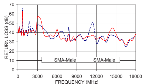
141-24SM+ RETURN LOSS
