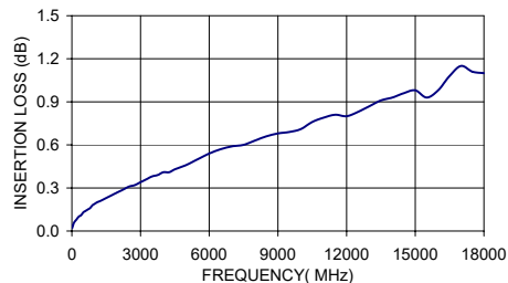
141-18SM+ INSERTION LOSS
