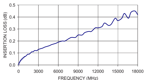
086-3SMRSM+ INSERTION LOSS
