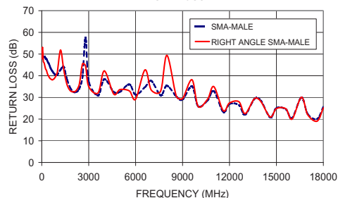
086-3SMRSM+ RETURN LOSS
