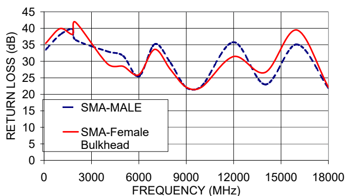
086-12BSM+ RETURN LOSS
