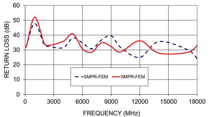
047-12SMPR+ RETURN LOSS
