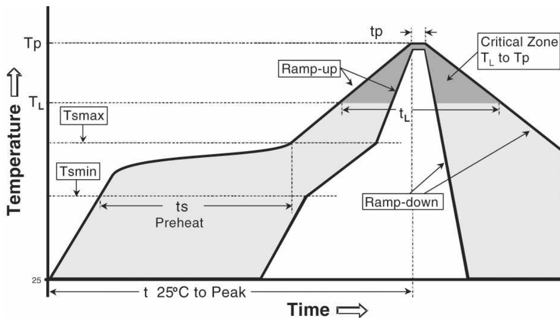
Figure 8 – Temperature profile.
