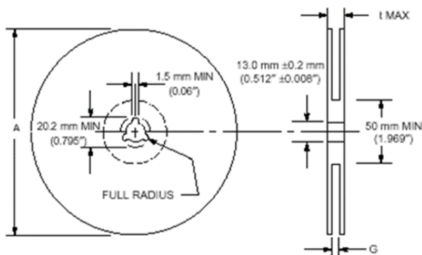
Figure 11 – Reel Dimensions and Capacity.
