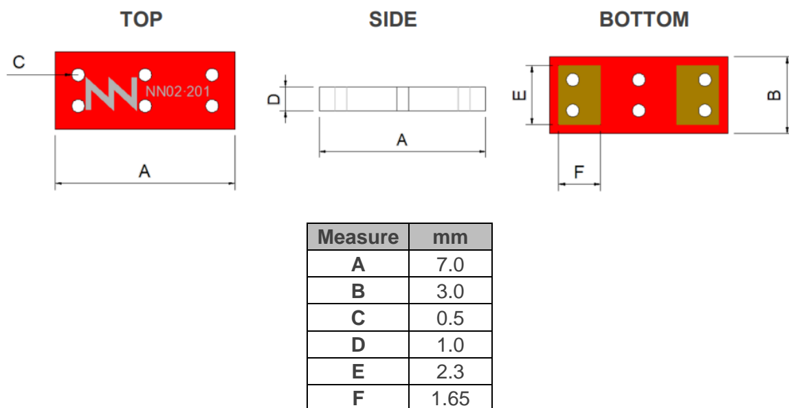
Figure 5 - ONE mXTEND™ antenna booster dimensions and tolerances
