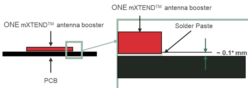
Figure 8 – Soldering Details.
