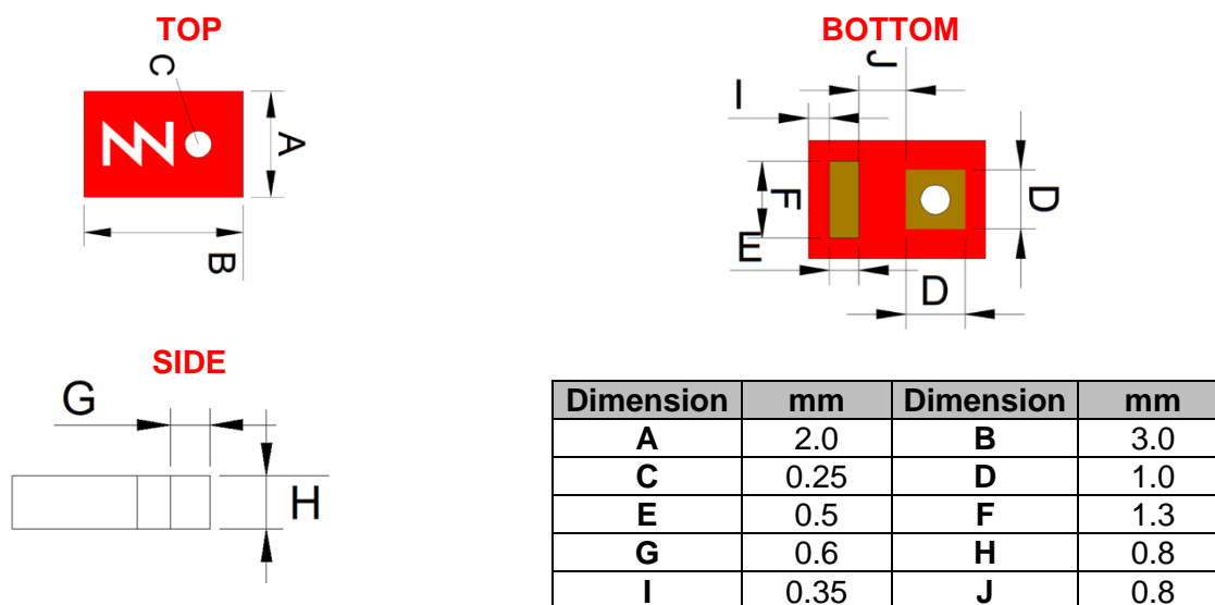
Figure 5 - NANO mXTEND ™ antenna booster dimensions and tolerances.
