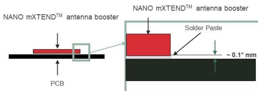
Figure 8 – Soldering Details.
