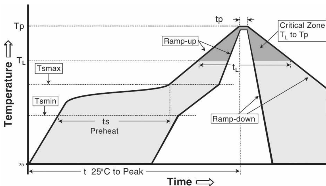
Figure 9 – Temperature profile.
