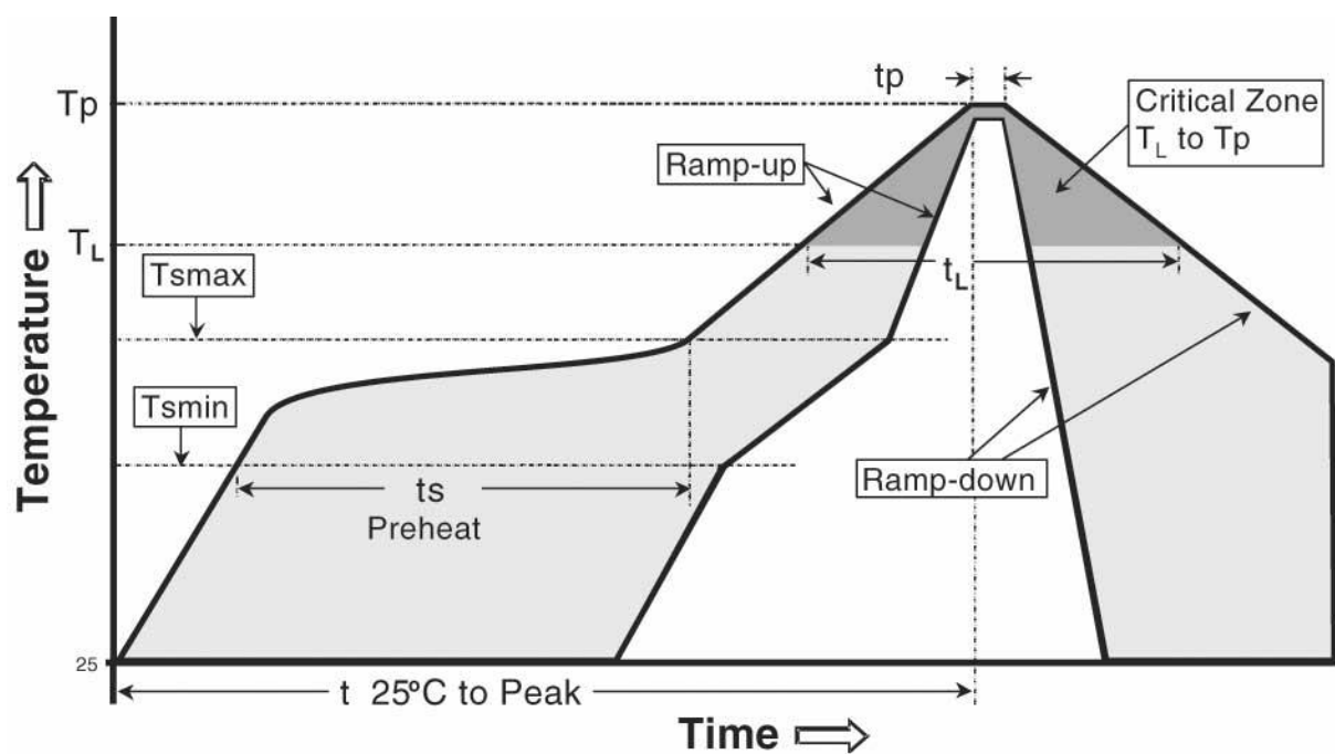
Figure 7 – Temperature profile.
