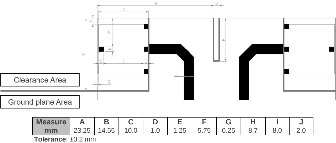
Figure 4 – Antenna Footprint Details
