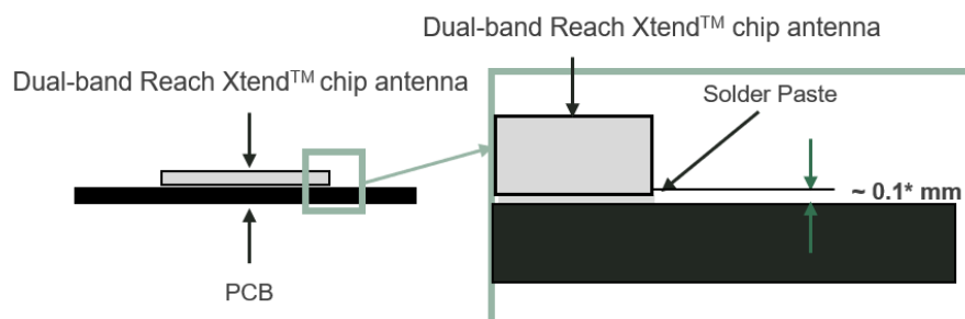
Figure 6 – Soldering Details.
