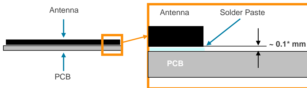
Figure 6 – Soldering Details.
