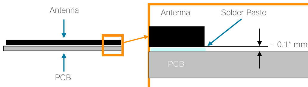
Figure 7 – Soldering Details.
