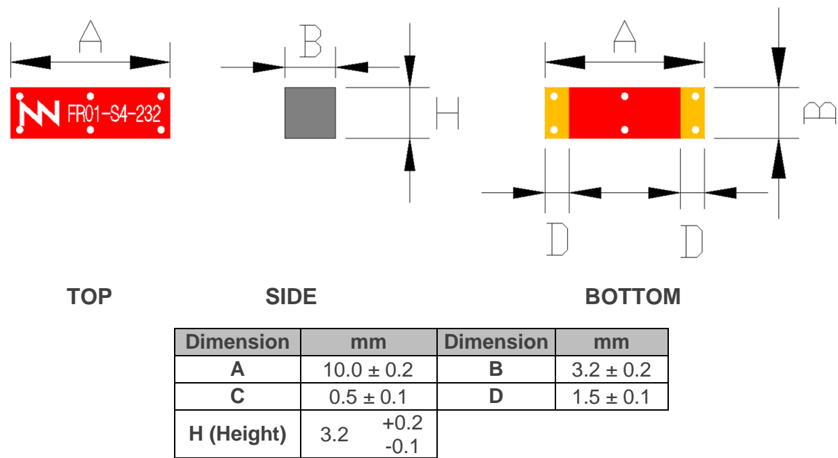
Figure 8 – BAR mXTEND™ Antenna Booster dimensions and tolerances.
