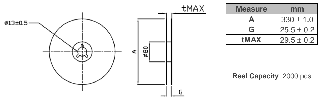
Figure 16 – Reel Dimensions and Capacity.
