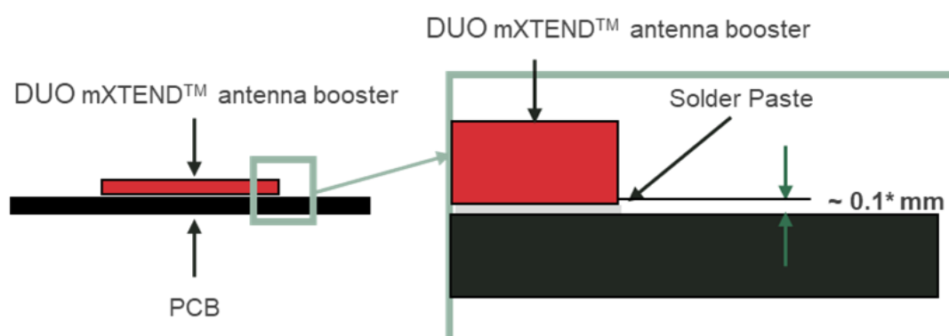
Figure 19 – Soldering Details.
