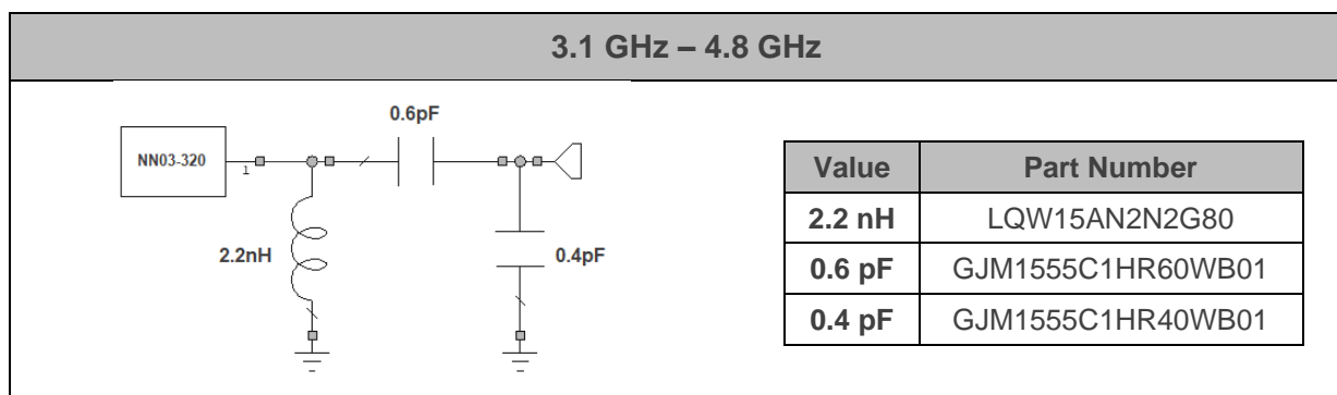
Figure 12 – Matching network implemented in the Evaluation Board (
