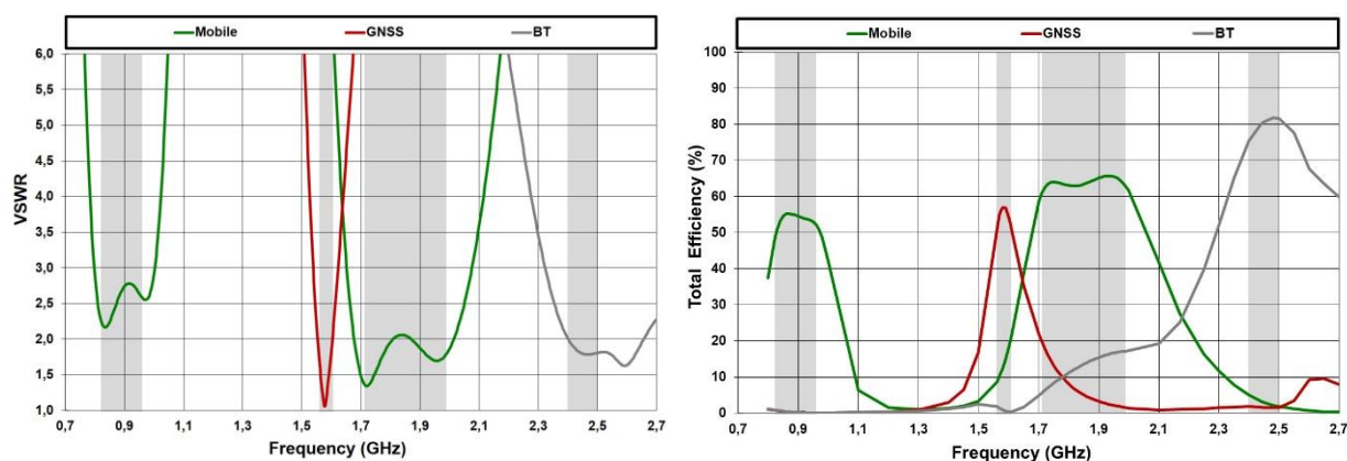
Figure 19 – VSWR and Total Efficiency for the different bands covered by the Evaluation Board from Figure 13. Simulated results obtained with CST.
