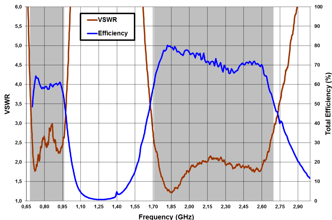
Figure 4 – VSWR and Total Efficiency for the 698 – 960 MHz frequency range and for the 1710 – 2690 MHz frequency range (from the Evaluation Board) ( Error! Reference source not found. ).
