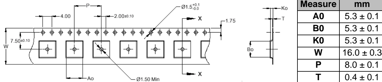
Figure 9 – Tape dimensions and Tolerances.
