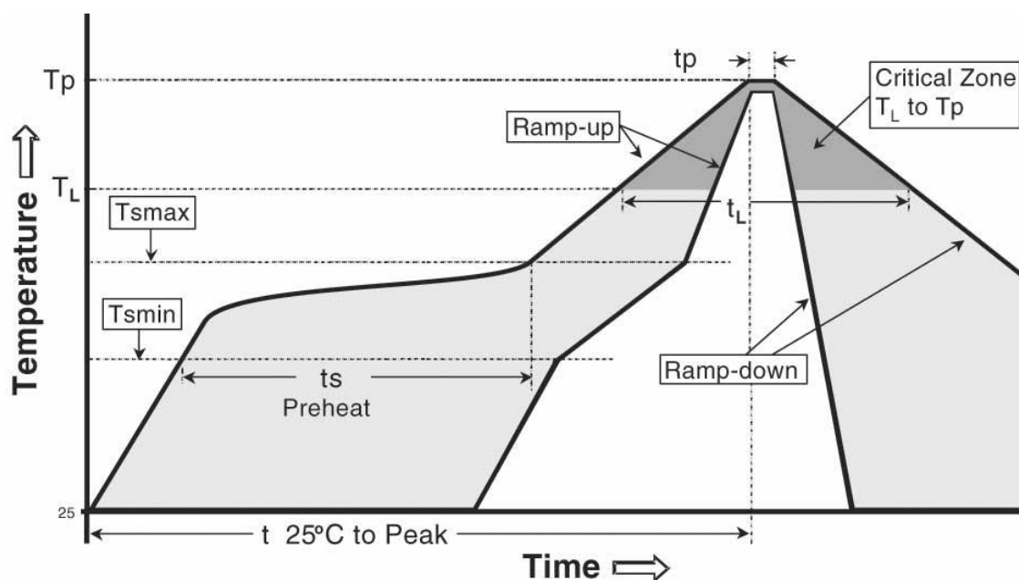
Figure 8 – Temperature profile.
