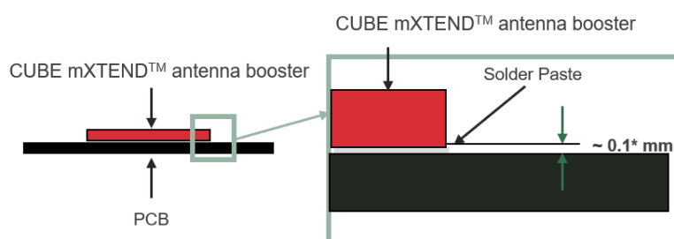
Figure 7 – Soldering Details.
