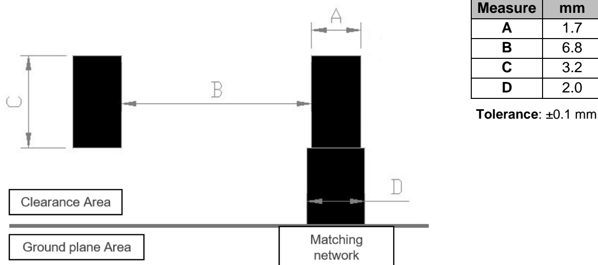
Figure 5 – Footprint dimensions for the single booster.
