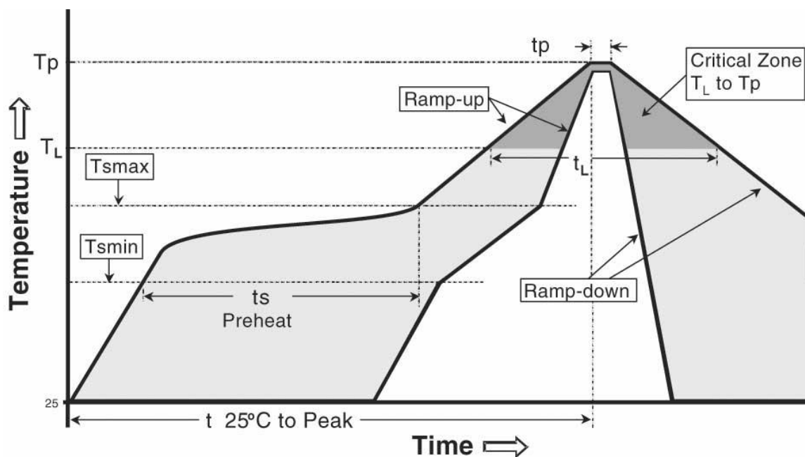
Figure 8 – Temperature profile.
