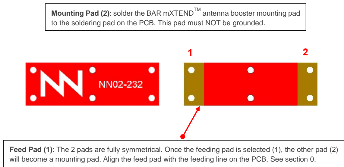
Figure 6 – Pads of the BAR mXTEND ™ antenna booster NN02-232
