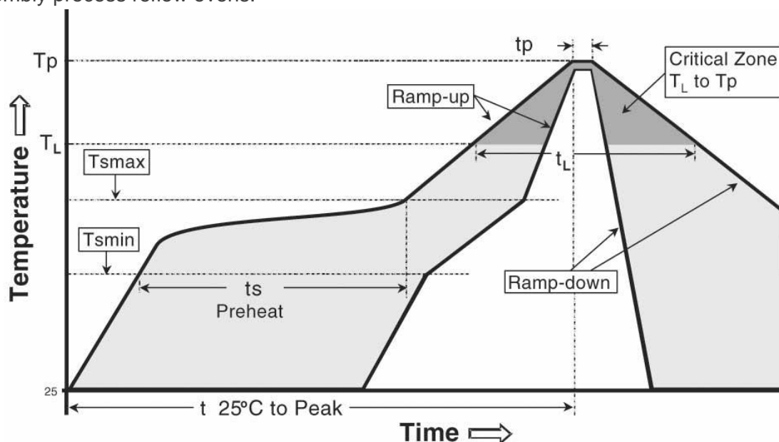
Figure 18 – Temperature profile.
