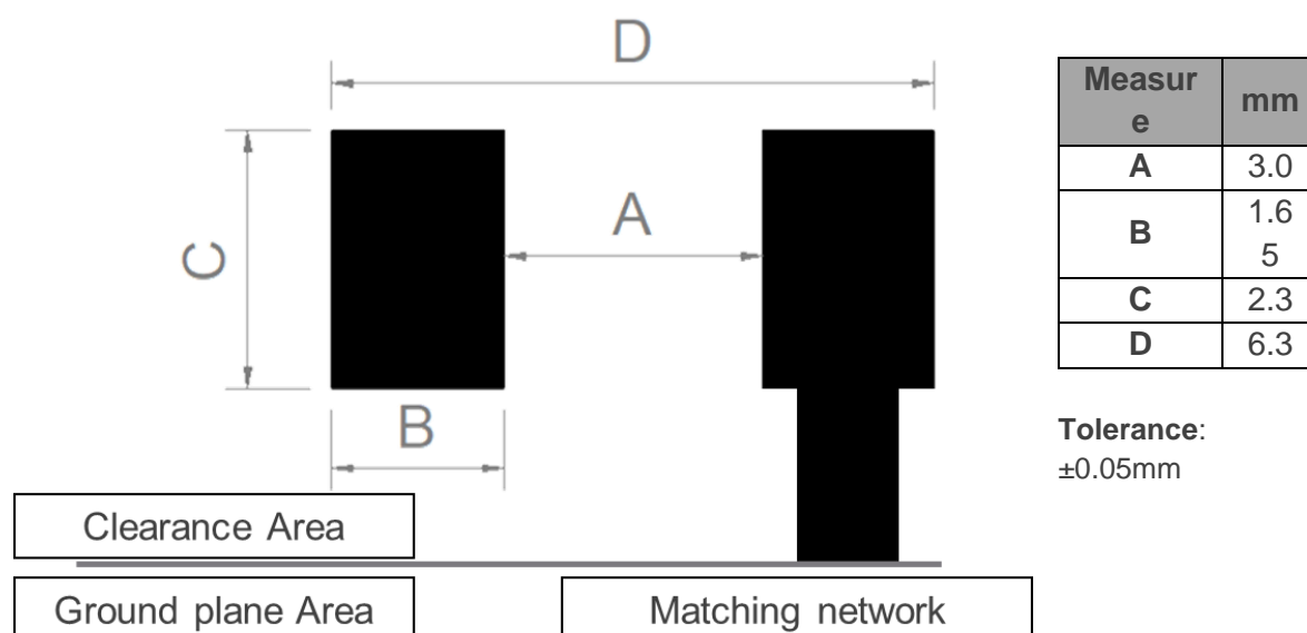
Figure 15 – Footprint dimensions for the ONE mXTEND ™ (NN02-201) antenna booster.
