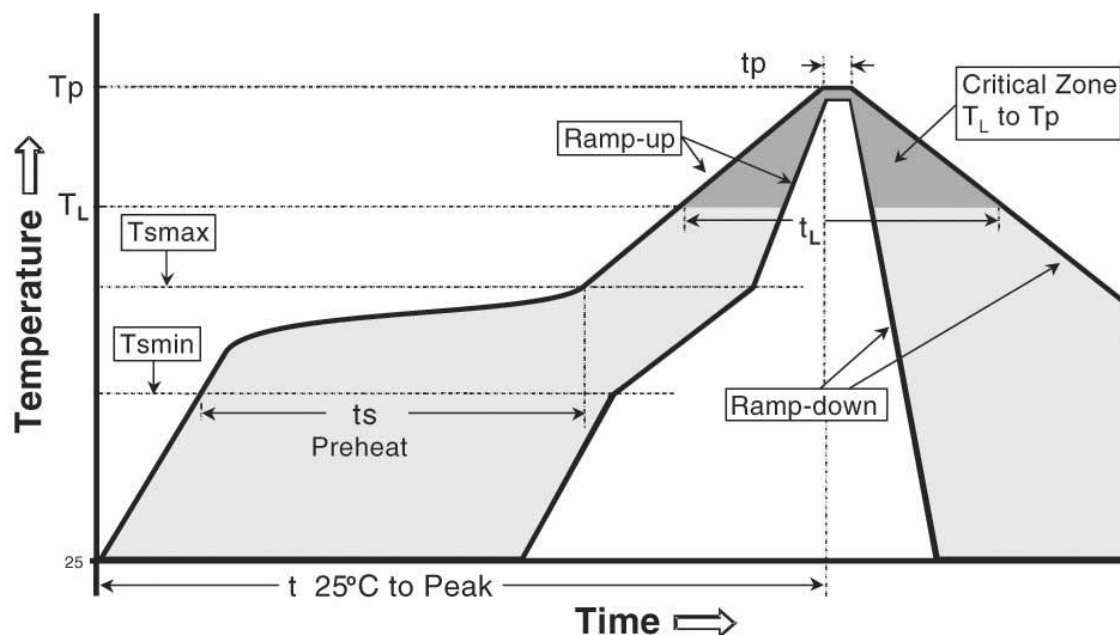
Figure 4 – Temperature profile.
