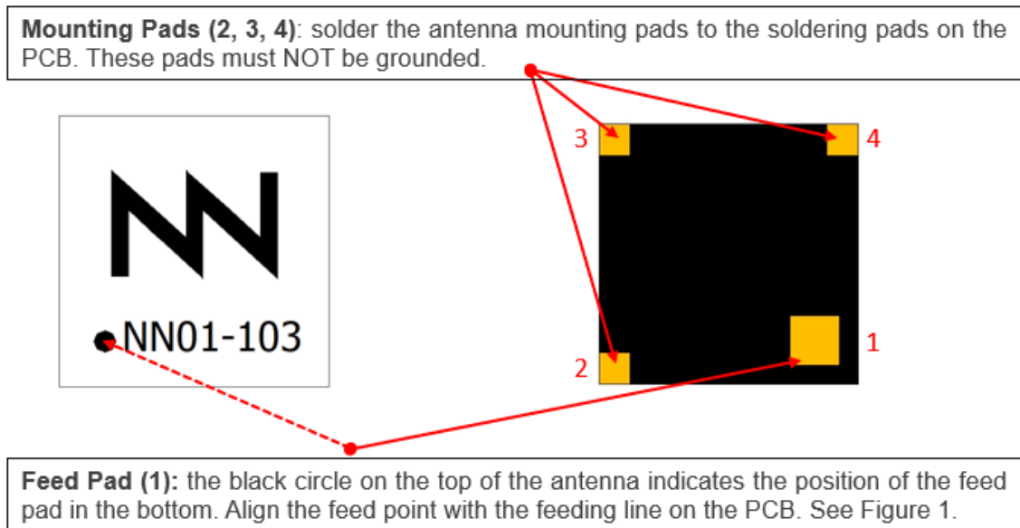
Figure 2 – Pads of the Geofind ™ chip antenna.
