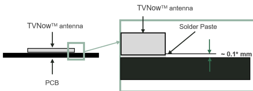
Figure 6 – Soldering Details.
