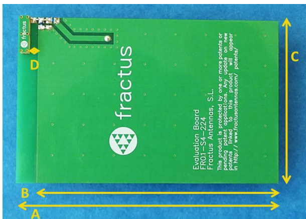
Figure 4 – EB_FR01-S4-224-CR80-2,4-5 in CR80 standard format. Evaluation Board providing operation from 2.4 GHz to 2.5 GHz and from 4.9 GHz to 5.875 GHz.
