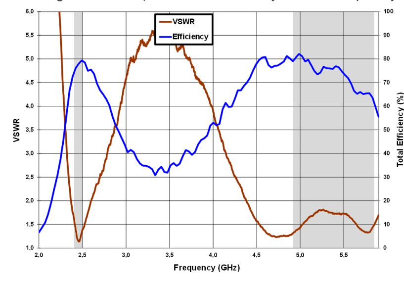
Figure 3 – VSWR and Total Efficiency for the 2.4 – 2.5 GHz frequency range and for the 4.9 – 5.875 GHz frequency range from the evaluation board (Figure 1).
