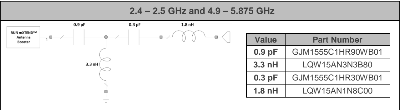
Figure 5 – Matching Network implemented in the evaluation board (Figure 4).
