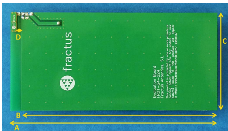
Figure 1 – EB_FR01-S4-224-2,4-5. Evaluation Board providing operation from 2.4 GHz to 2.5 GHz and from 4.9 GHz to 5.875 GHz.
