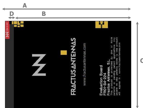
Figure 4 – EB_FR01-S4-224-CR80-1561-1606 in CR80 standard format. Evaluation Board providing operation for BeiDou E1 band (1561 MHz), GPS L1 band (1575 MHz) and for GLONASS L1 band (from 1598 MHz to 1606 MHz).
