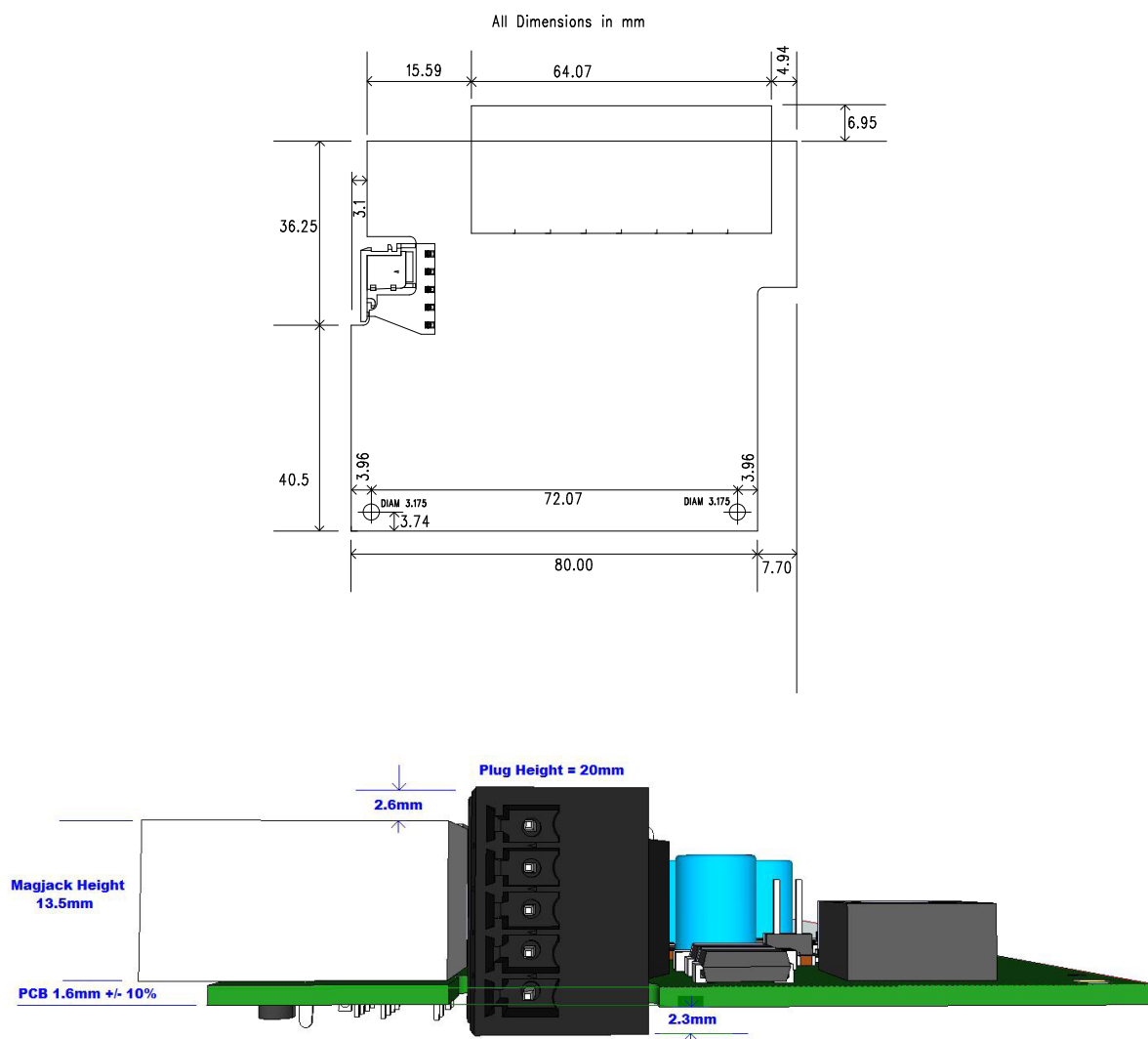
Power Terminal Pin Outs
