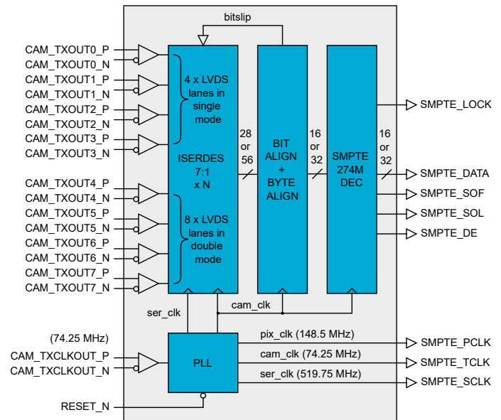
Figure 1: Sony LVDS camera interface (internal architecture)
