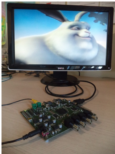
Figure 11: Photo of the test setup
