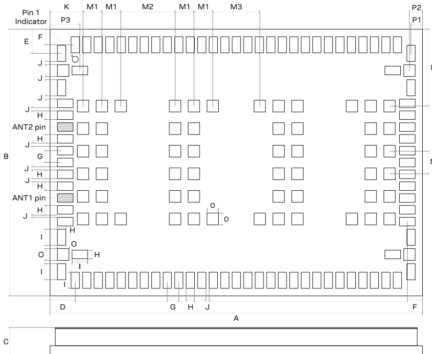
Figure 3: TOBY-L2 series dimensions (bottom and side views)
