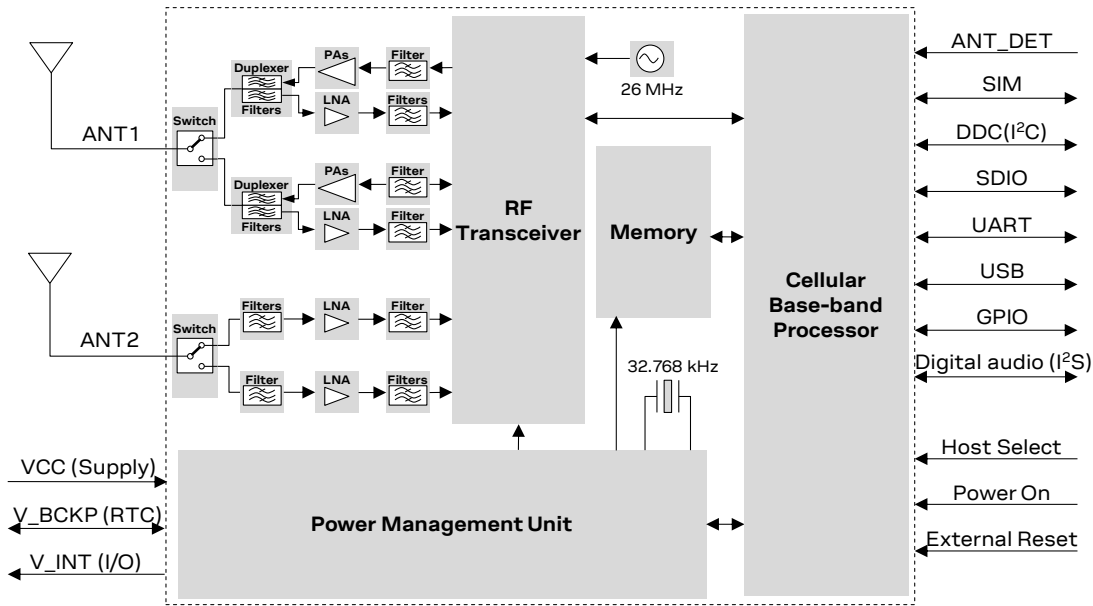
Figure 1: TOBY-L2 series block diagram
