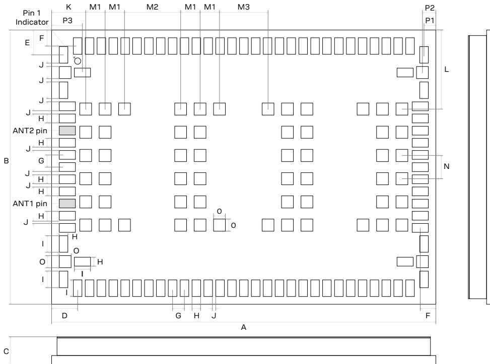
Figure 3: TOBY-L2 series dimensions (bottom and side views)
