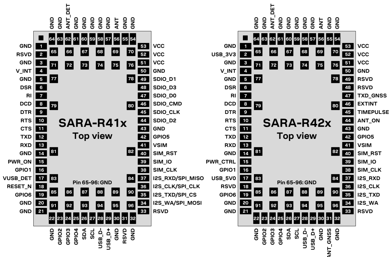
Figure 4: SARA-R4 series pin assignment (top view)
