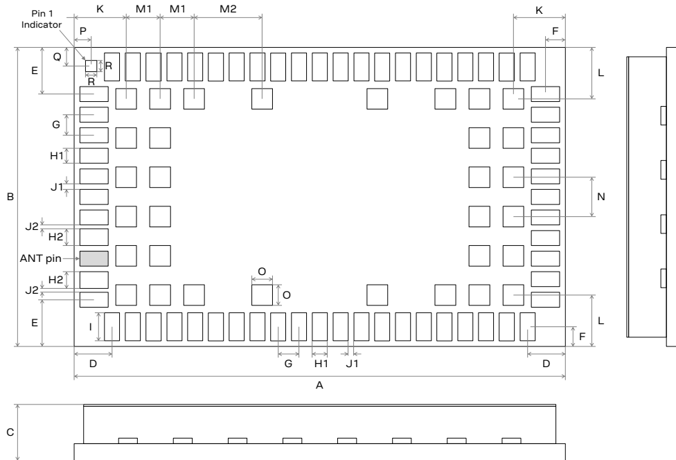
Figure 3: SARA-G450 module dimensions (bottom and sides views)
