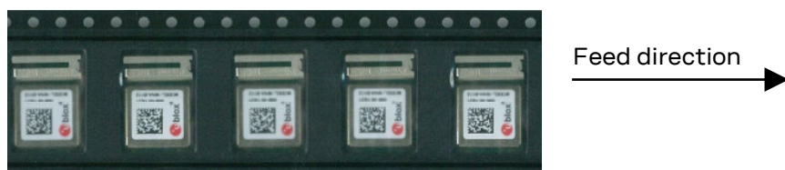
Figure 11: Orientation of NINA-W132 module on tape
