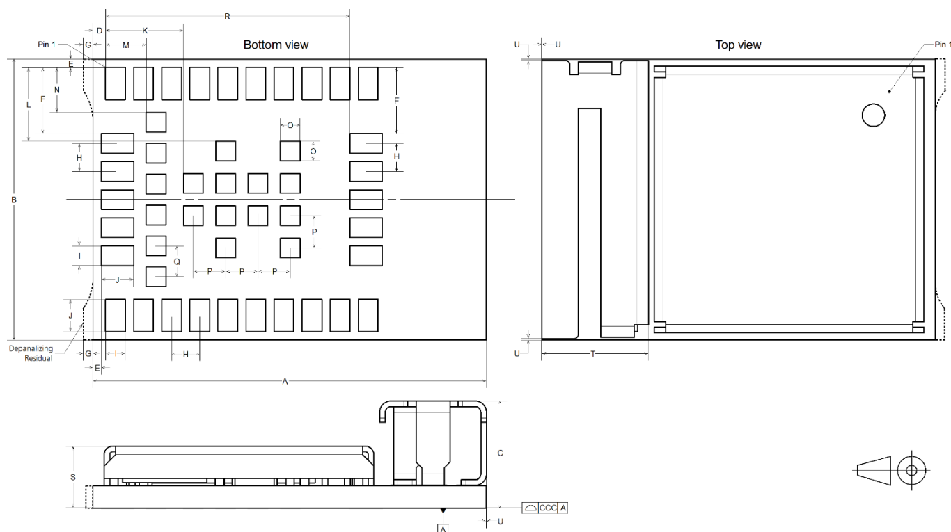
Figure 7: NINA-W132 mechanical outline
