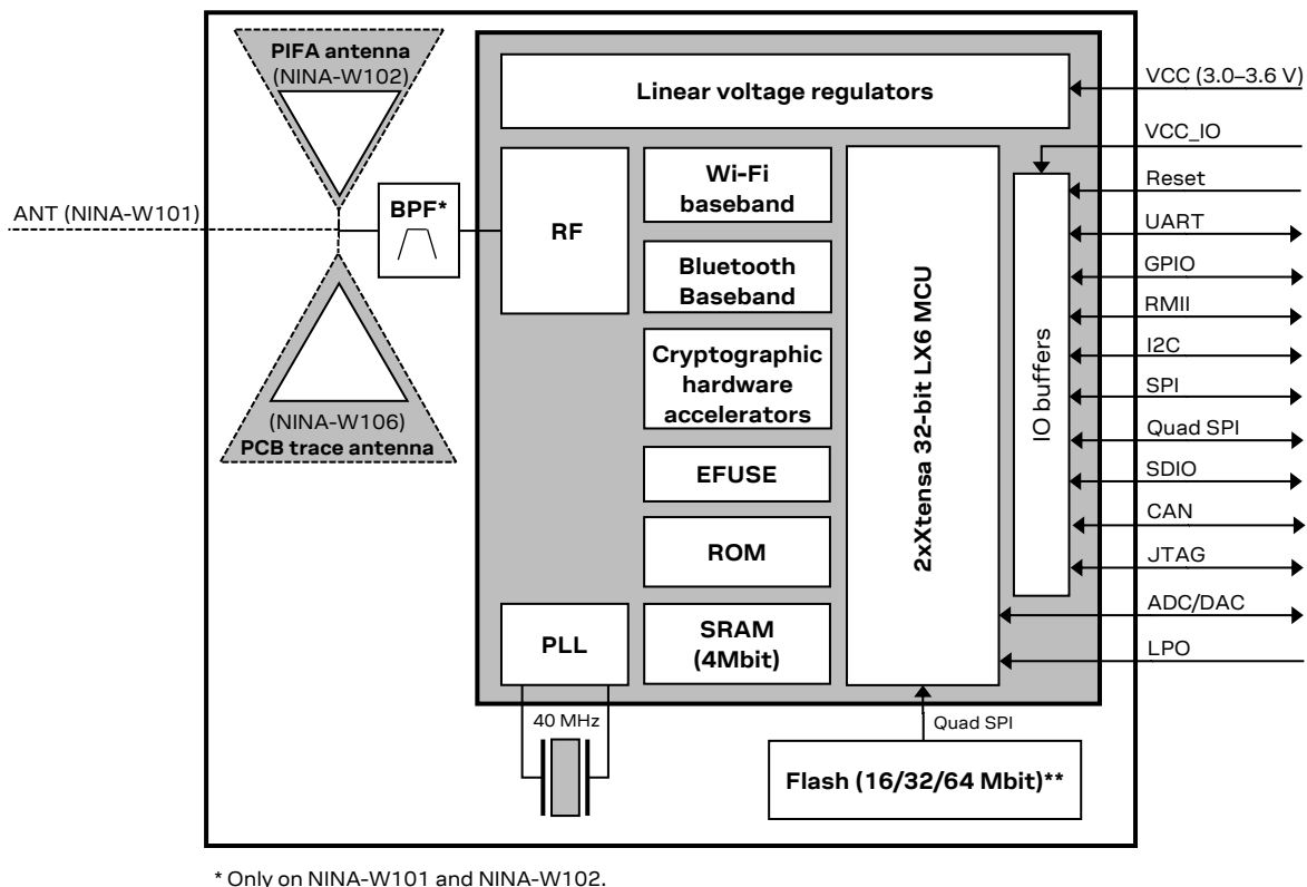
Figure 1: NINA-W10 series block diagram
