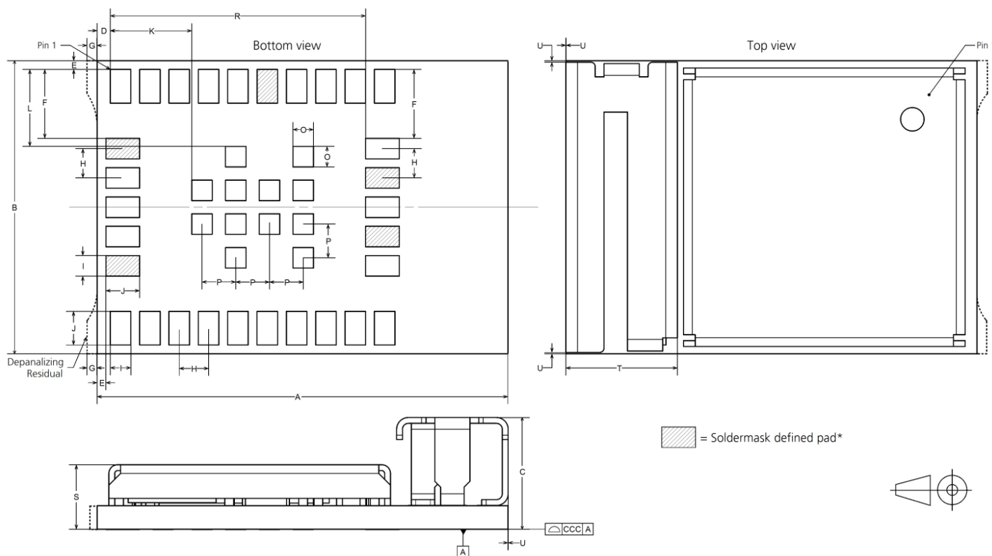
Figure 10: NINA-B112 mechanical outline
