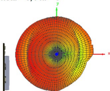
Theta = 0, Phi = 0
