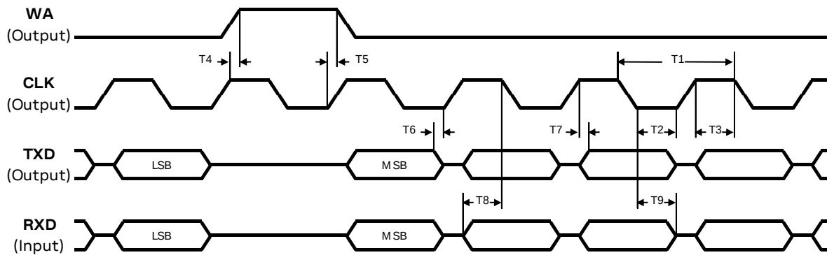
Figure 10: AC characteristics of digital audio interface in PCM mode ( \langle I2S\_mode \rangle = 1 ) and host mode enabled
