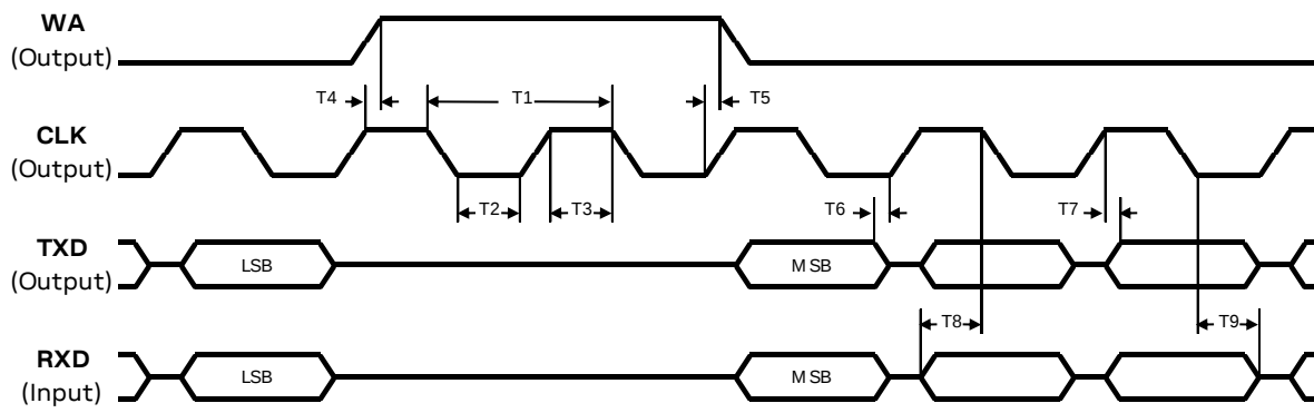
Figure 9: AC characteristics of digital audio interface in PCM mode ( \langle I2S\_mode \rangle = 0 ) and host mode enabled
