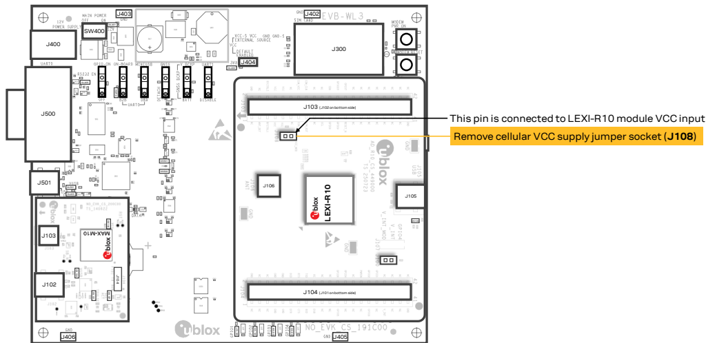
Figure 10: Jumper socket to be removed for LEXI-R10 module's current consumption measurement on EVK-R10 new model
