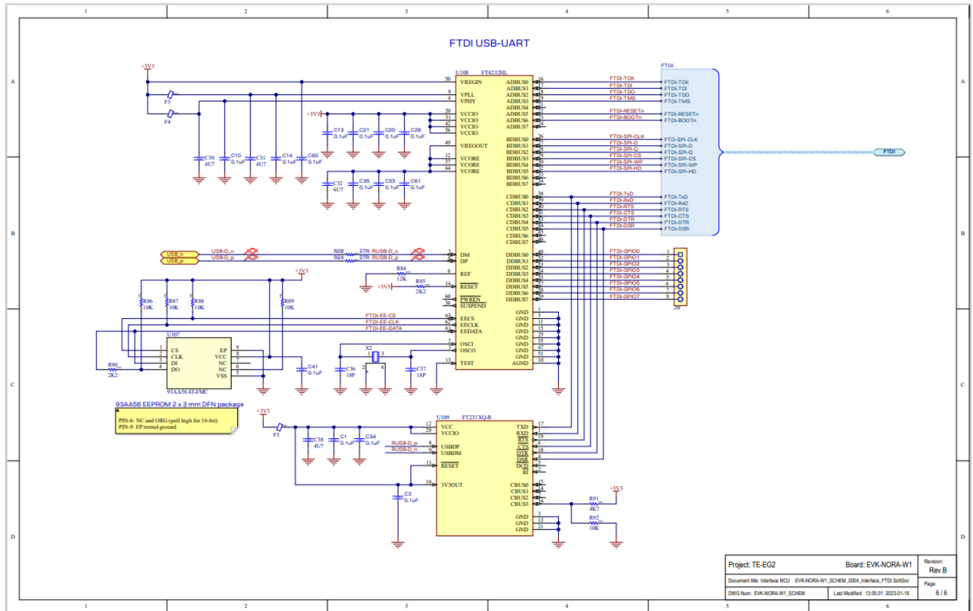
Figure 25: Interface FTDI
