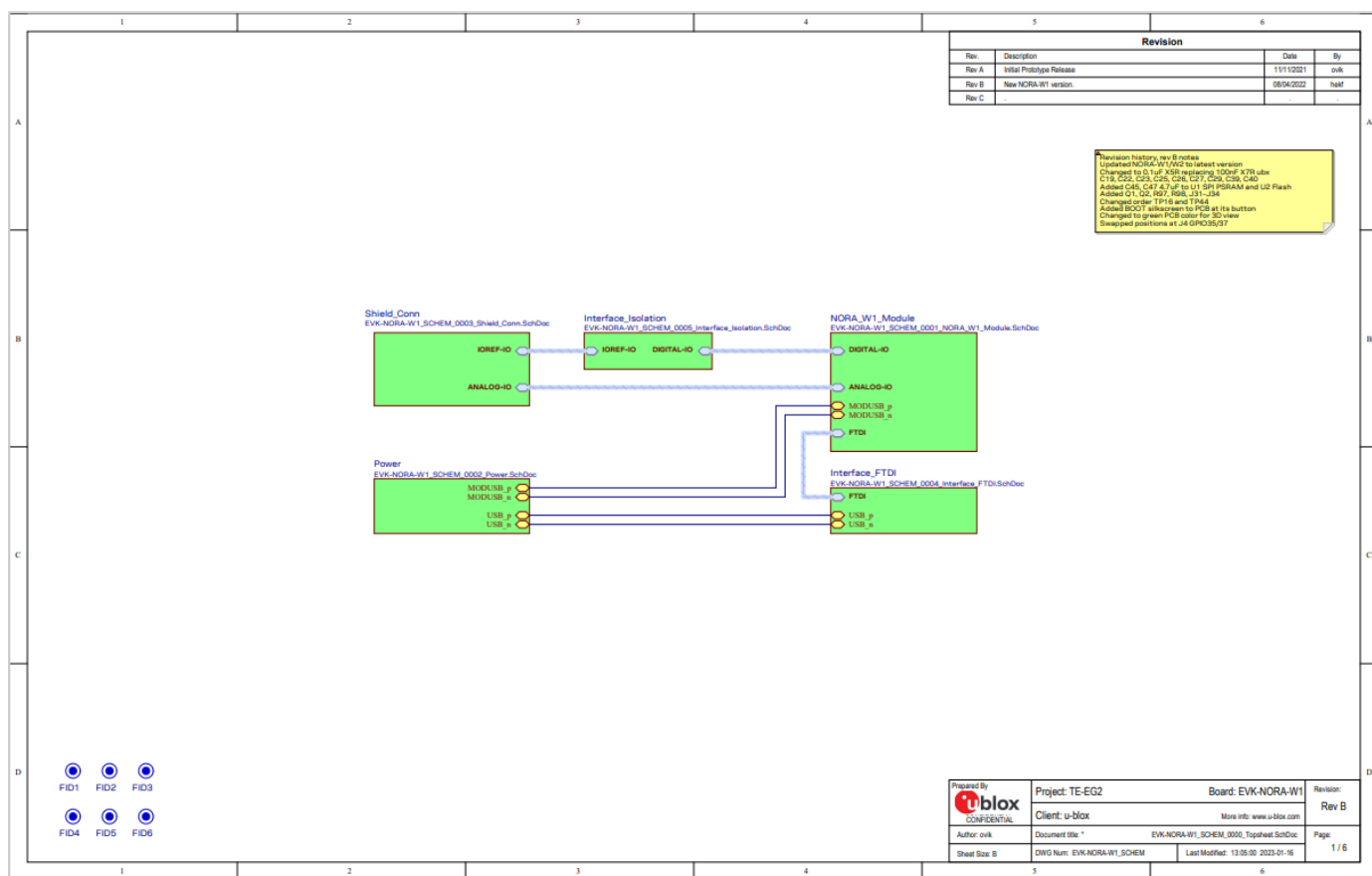
Figure 20: Top page
