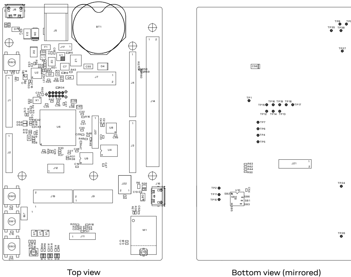
Figure 22: Component layout
