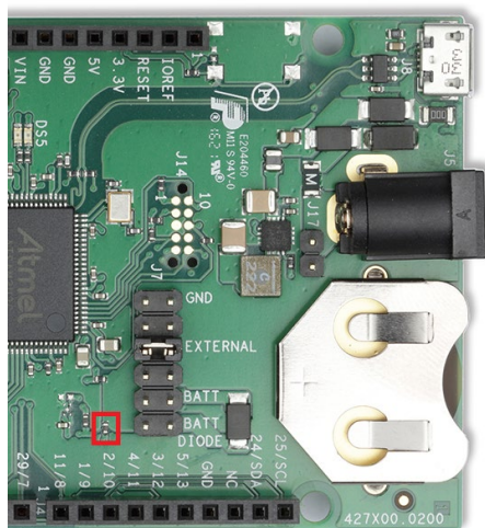
Figure 5: Resistor R9
