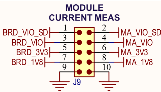
Figure 7: MAYA-W1 current measurement (J9)
