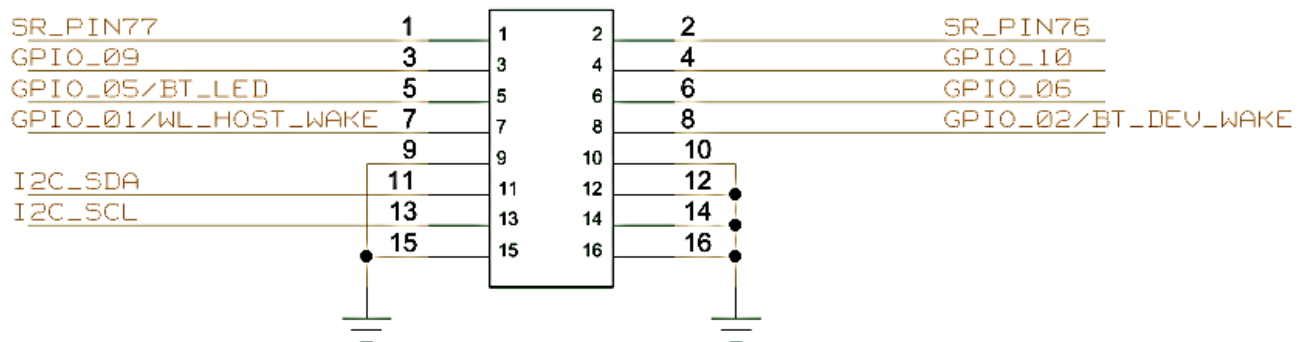
Figure 20: Connector J303
