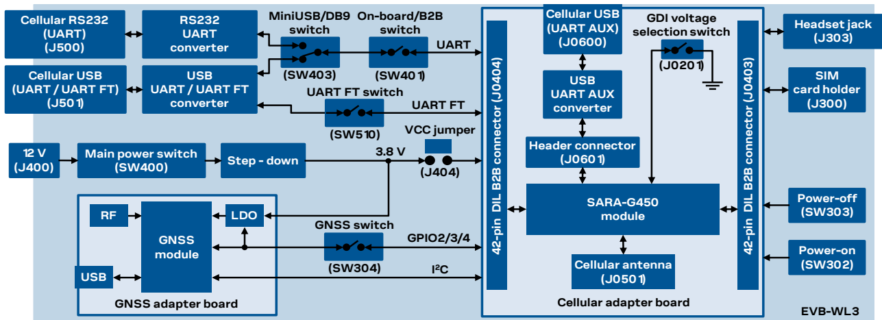
Figure 2: Block diagram of EVK-G45
