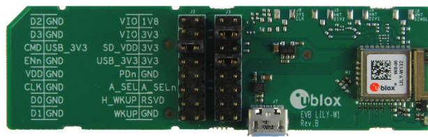
Figure 2: EVK-LILY-W132 evaluation kit
