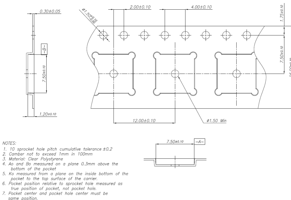
Figure 6: EVA-M8M/Q tape dimensions
