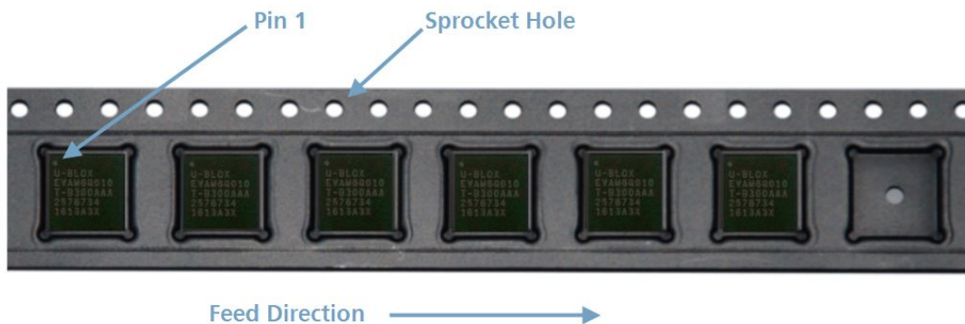
Figure 5: Orientation of EVA-M8Q modules on the tape
