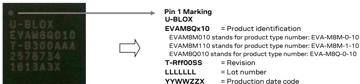
Figure 7: Description of EVA-M8Q product label
