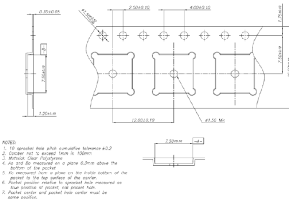
Figure 6: EVA-M8M tape dimensions
