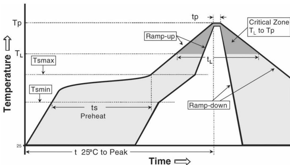
Figure 19: Reflow profile
