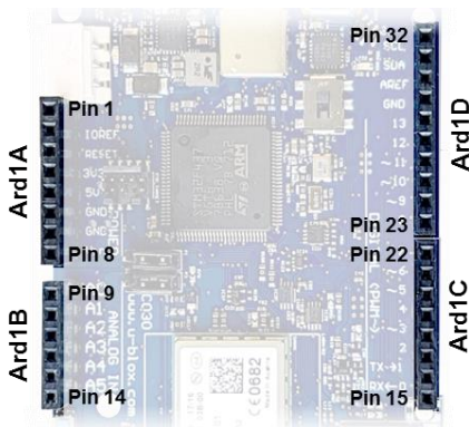
Figure 18: C030 Arduino™ UNO R3 connectors
