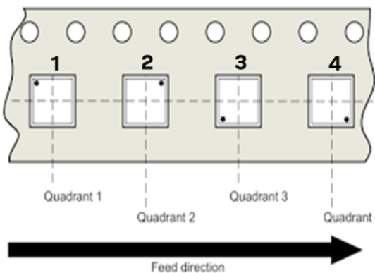
Figure 22: Carrier tape quadrants
