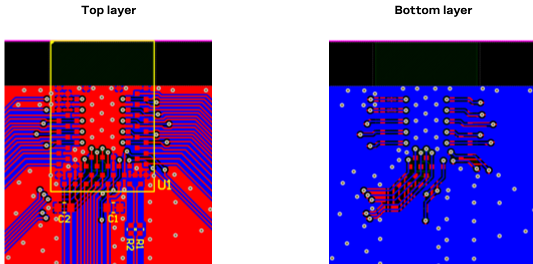
Figure 6: BMD-340 two-layer fan-out example
