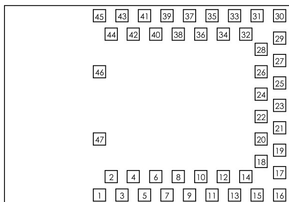
Figure 2: BMD-300 pin assignment (top view)
